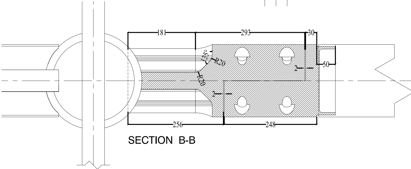
SECTION B-B
